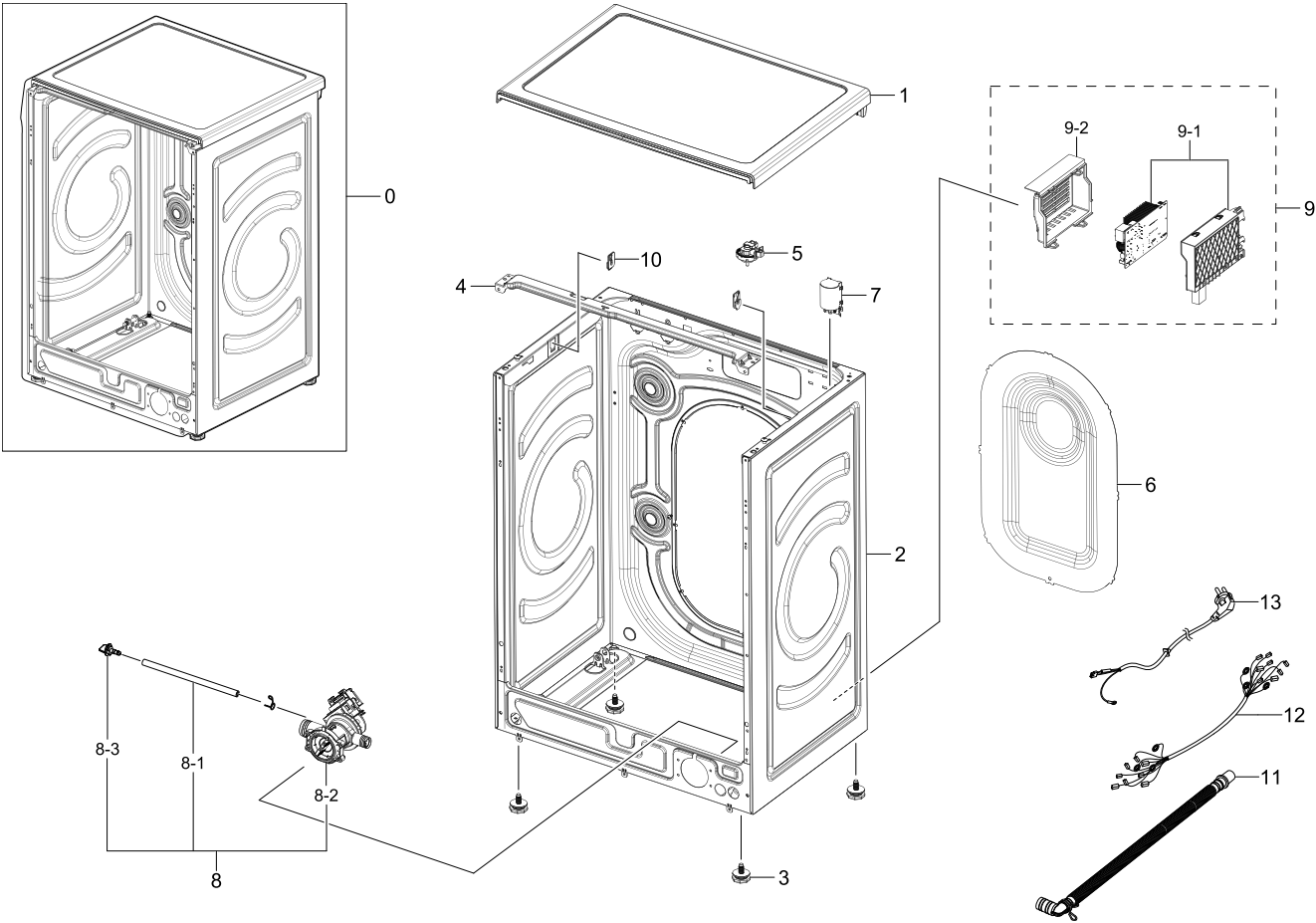
Exploded View
