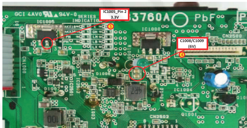
Main PCB
