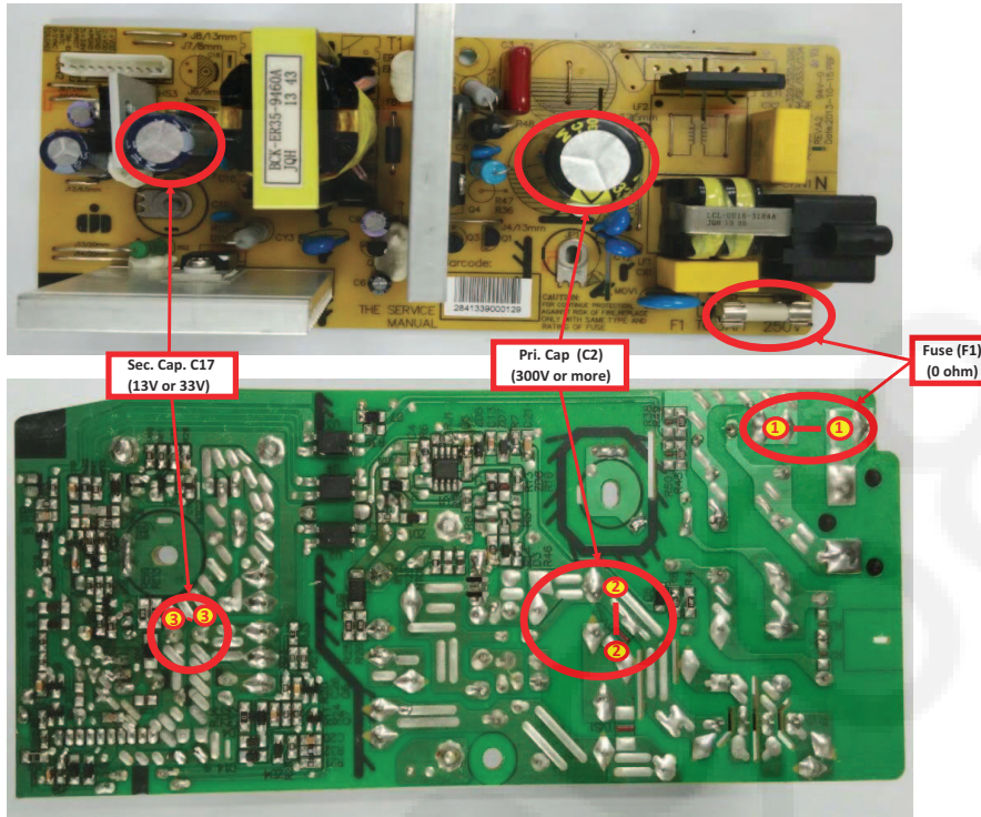
Main PCB
